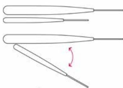
K125 AND K70 JUMPING HILL POSITION ADAPTATION TO EXISTING SKIING HILLS
